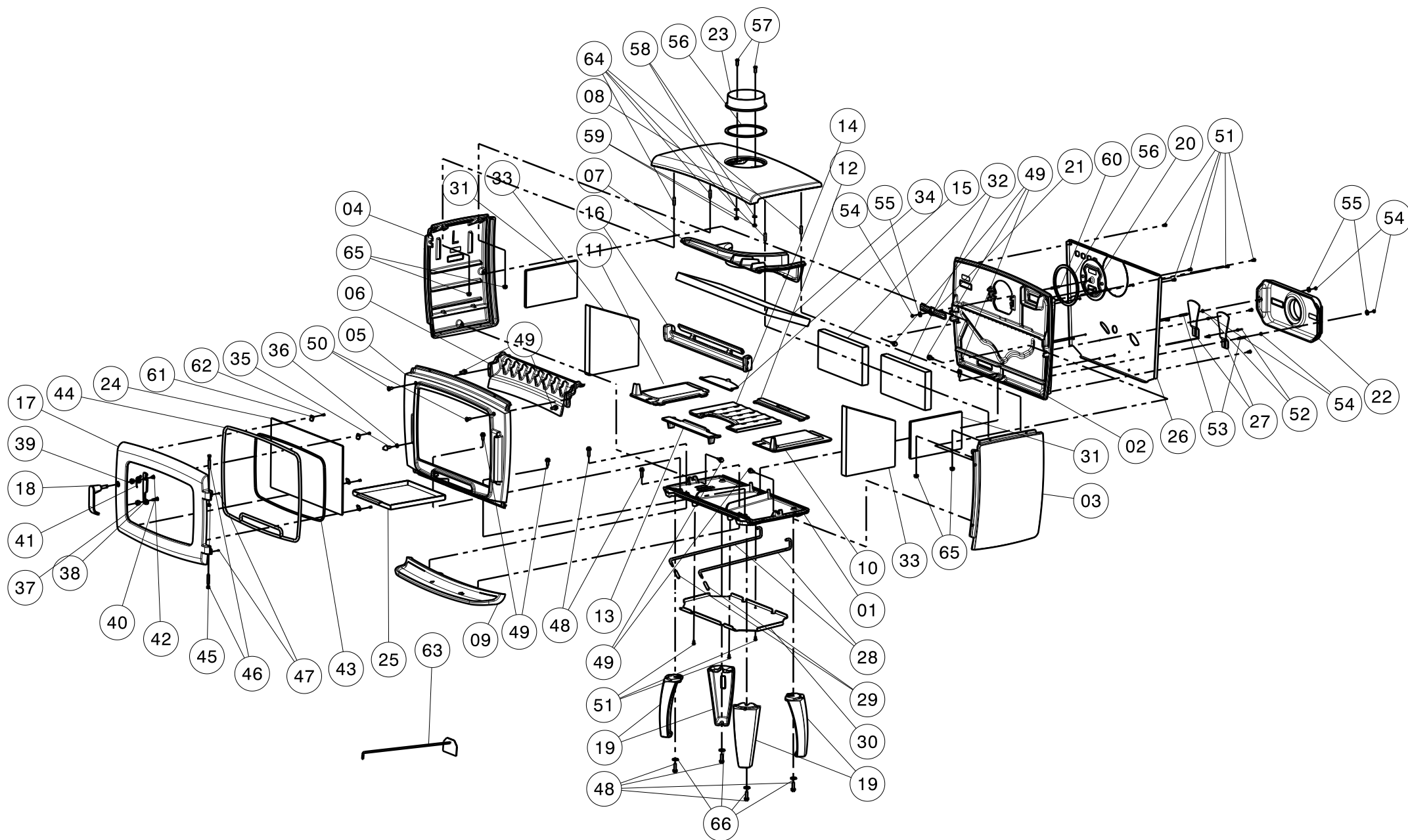
Exploded view Scale: 1:20
